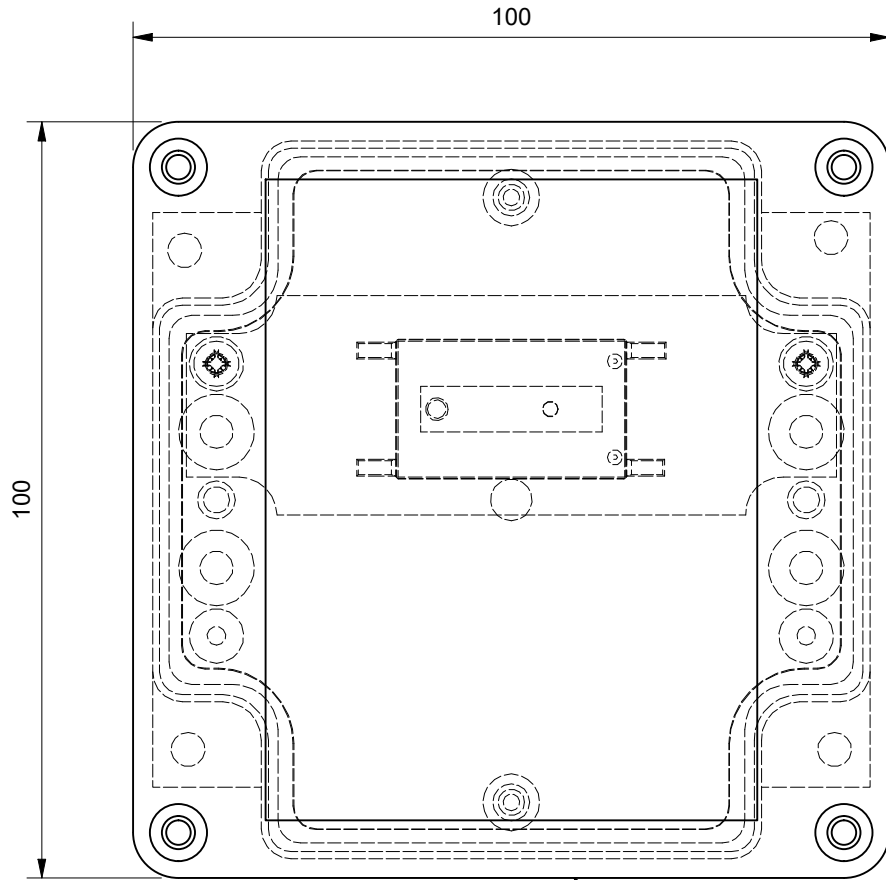
GREY POLYCARBONATE ENCLOSURE WITH CLEAR LID
