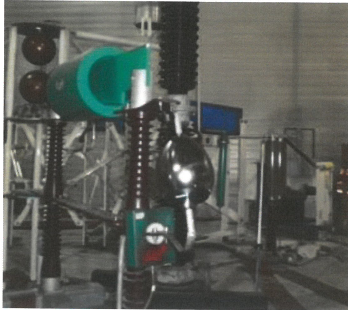
Figure 3. Electric Test.
